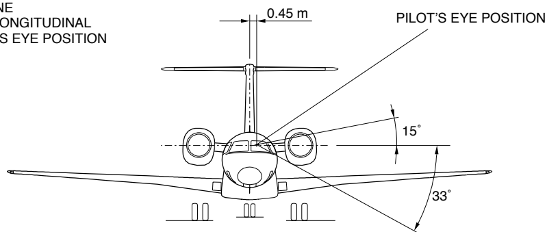
Figure 4.4.1 - Visibility from Cockpit in Stationary Position
