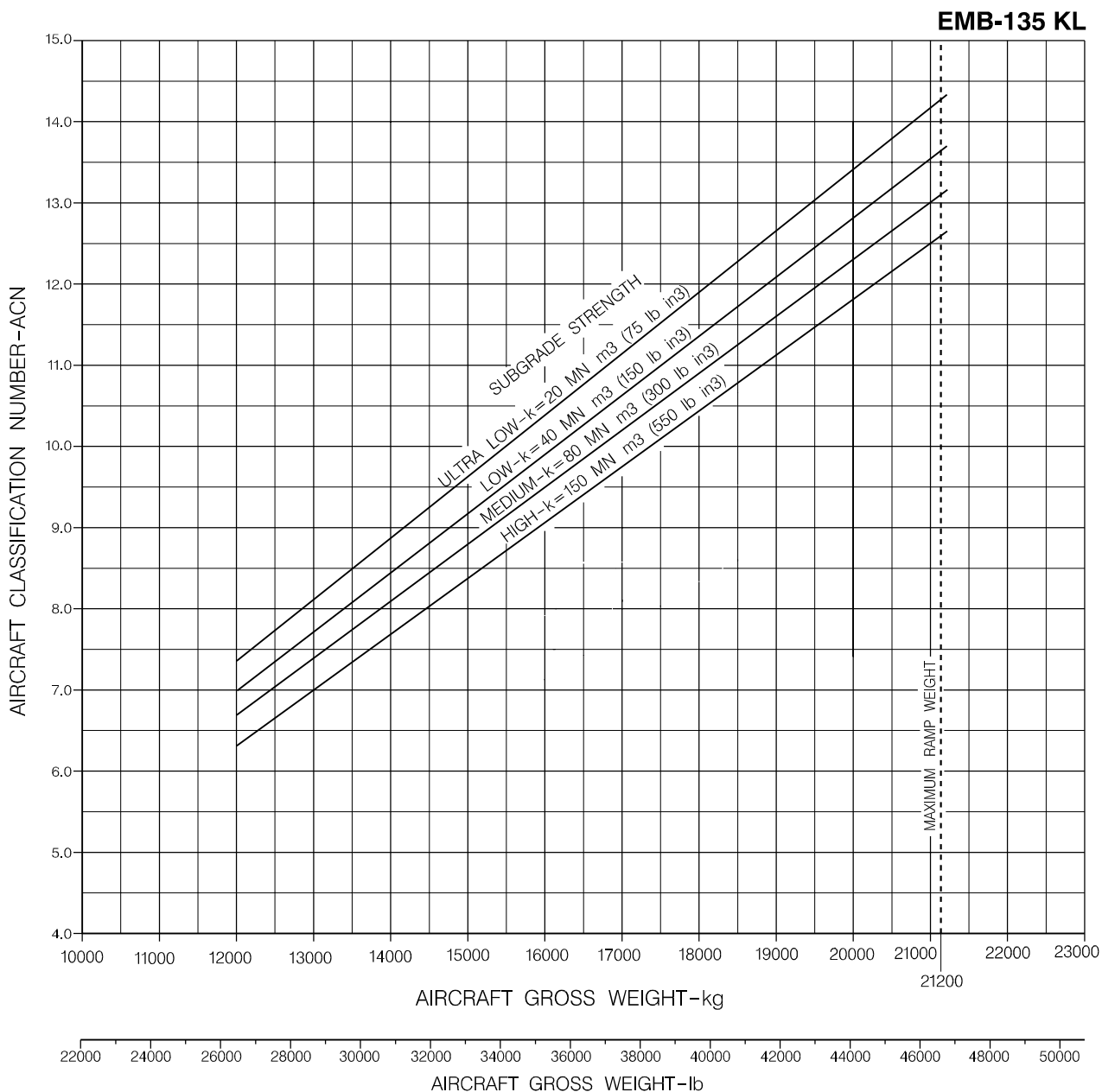
Figure 7.9.2 - Aircraft Classification Number Rigid Pavement Sheet 2
