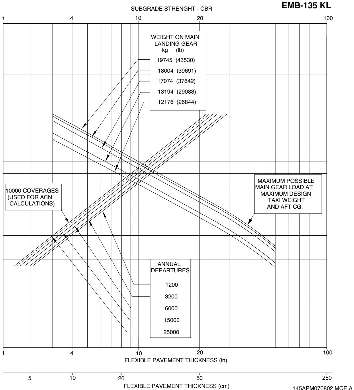
Figure 7.5.1 - Flexible Pavement Requirements - U.S. Army Corps of Engineers Design Method Sheet 2
