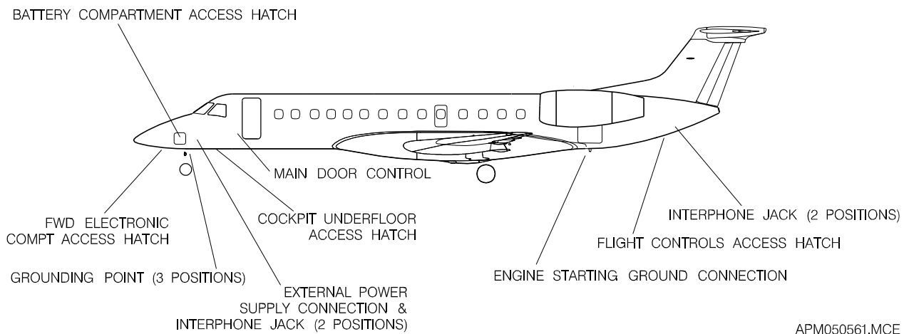
Figure 5.4.2 - EMB-135 KL Ground Servicing Connections
