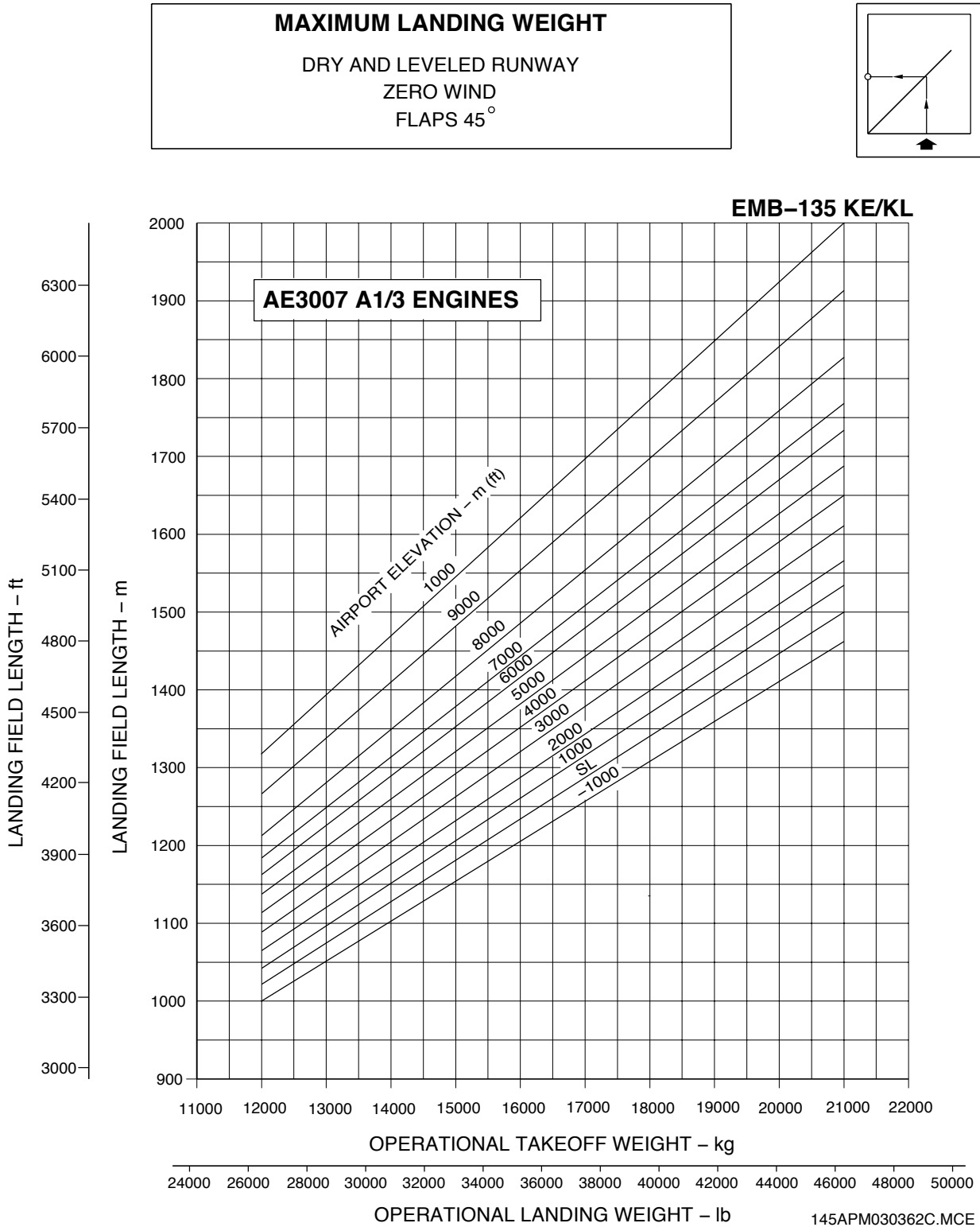
Figure 3.4.1 - FAR Landing Runway Length Requirements - Flaps 45°
