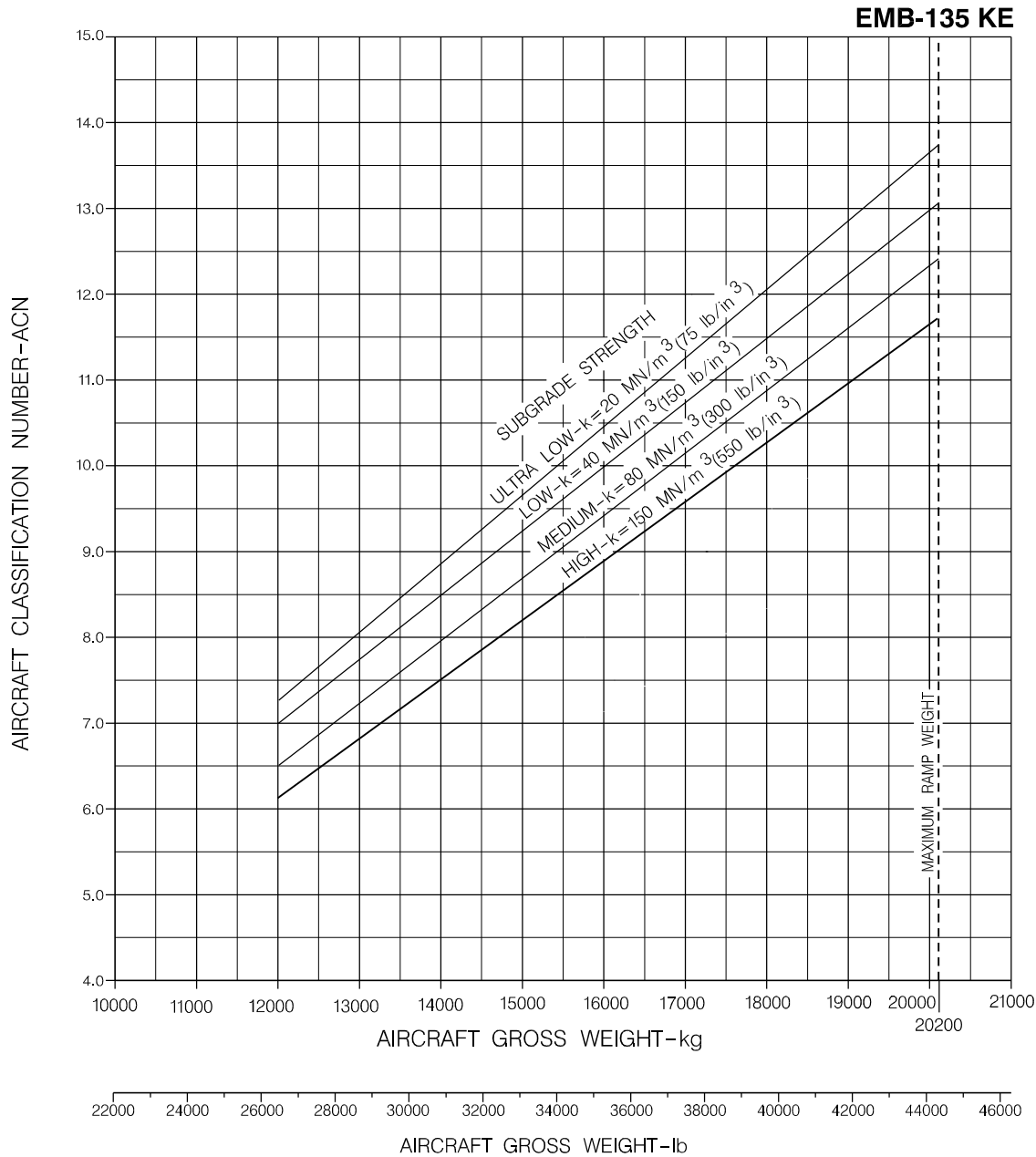
Figure 7.9.2 - Aircraft Classification Number Rigid Pavement Sheet 1
